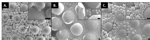
Figure 2. mCC structures created by sonication on a flat glass substrate. Triphasic mixtures were made from A) 0.6, 18, and 100 \mu\text{m} particles, B) 1, 10, and 100 \mu\text{m} particles, and C) 6, 18, and 100 \mu\text{m} particles. All scale bars are 10 \mu\text{m} .
